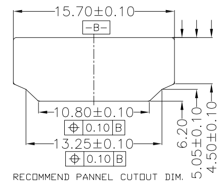
RECOMMEND PANNEL CUTOUT DIM.
